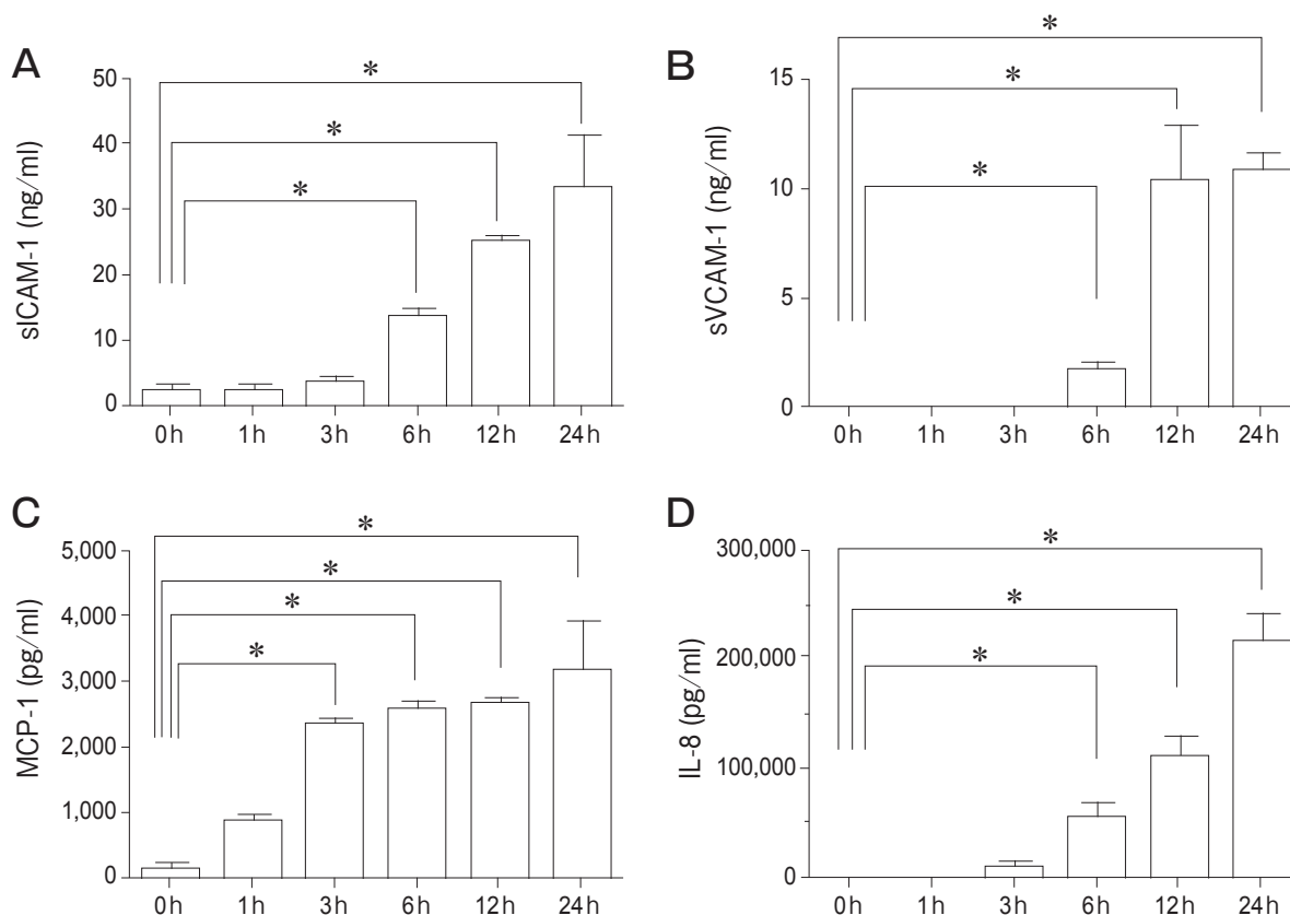
Fig. 6 Effects of \text{TNF-}\alpha + \text{IL-1}\beta on the secretion of sICAM-1, sVCAM-1, MCP-1, and IL-8 in human PMVEC. Treatment with \text{TNF-}\alpha + \text{IL-1}\beta (10 ng/ml) for 6 h significantly increased the secretion of sICAM-1 (A), sVCAM-1 (B), and IL-8 (D). The secretion of MCP-1 (C) was increased by stimulation for 3 h. Data are presented as mean \pm SD ( n = 4 in each group). * p < 0.05 in comparison with 0 h in each group. sICAM-1, soluble intercellular adhesion molecule-1; sVCAM-1, soluble vascular cell adhesion molecule-1; MCP-1, monocyte chemoattractant protein-1; IL-8, interleukin-8.
