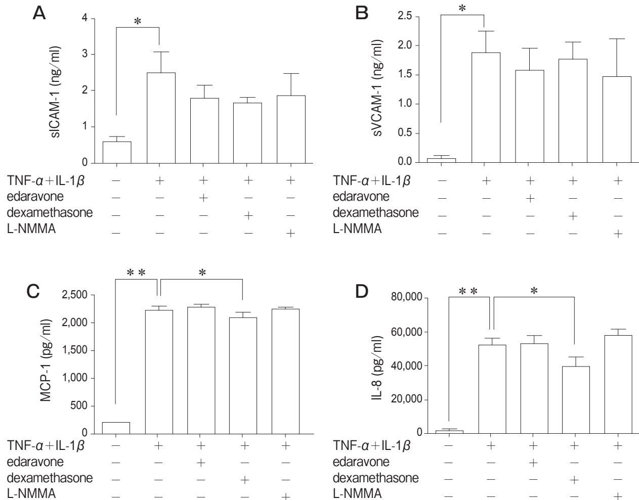
Fig. 7 Effects of edaravone, dexamethasone, and N-monomethyl-L-arginine (L-NMMA) on the secretion of sICAM-1, sVCAM-1, MCP-1, and IL-8 in the human PMVEC stimulated with TNF- \alpha + IL-1 \beta (10 ng/ml in both). Up-regulation of sICAM-1 and sVCAM-1 were not suppressed by these chemicals. MCP-1 and IL-8 were suppressed significantly by pretreatment with dexamethasone. Data are presented as mean \pm SD ( n=4 in each group). * p < 0.05 , ** p < 0.01 . sICAM-1, soluble intercellular adhesion molecule-1; sVCAM-1, soluble vascular cell adhesion molecule-1; MCP-1, monocyte chemoattractant protein-1; IL-8, interleukin-8.
